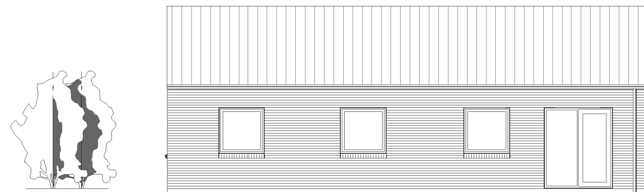
Facade mod vest 1 : 100
